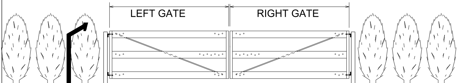
3'-6" HIGH DOUBLE 3 RAIL GATE KIT EXTERIOR ELEVATION
